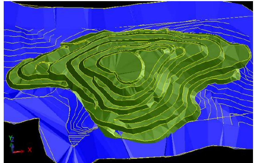
Dump Designing
